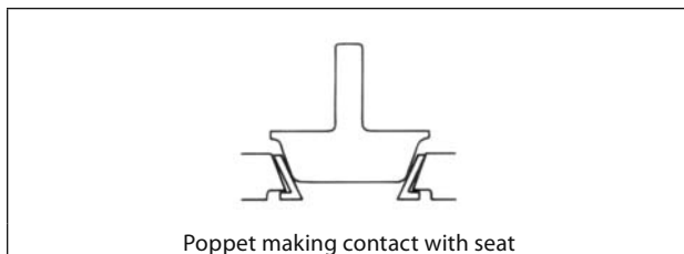
Poppet making contact with seat
