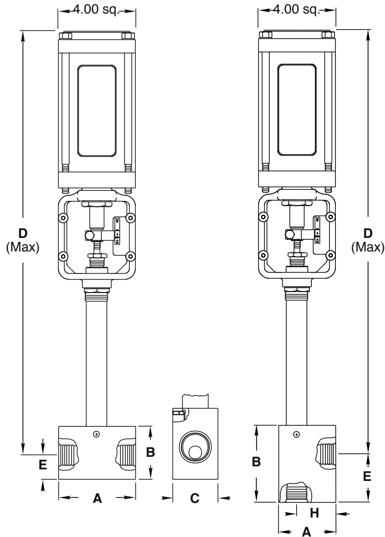
Globe Dimensions (inches): CES60 & CES12 Series
