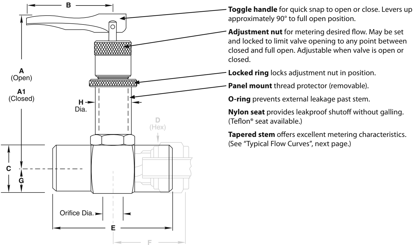
TM9400 Series Dimensions (inches)
