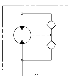
C Bi-Rotational Check Valves
