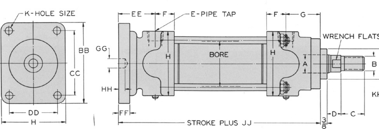
Model T754 - Blind Flange Mount
