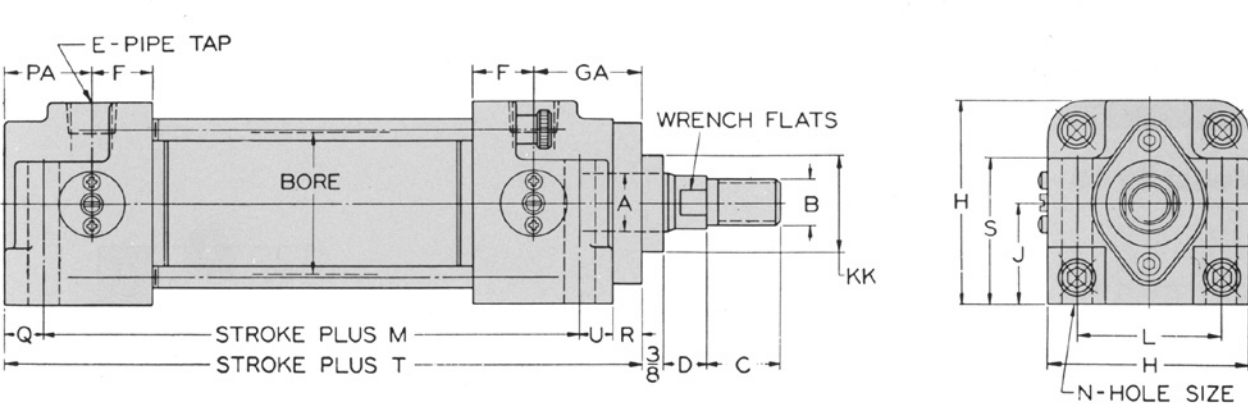
Model T753 - Rod Flange Mount
