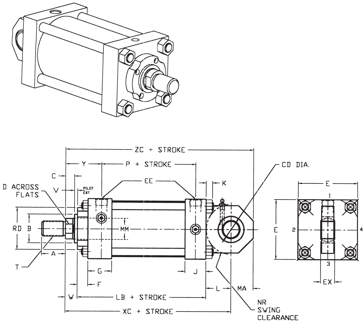
These Dimensions Are Constant Regardless of Rod Diameter
