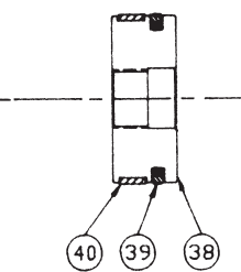
3L STANDARD PISTON (Codes G or H)
