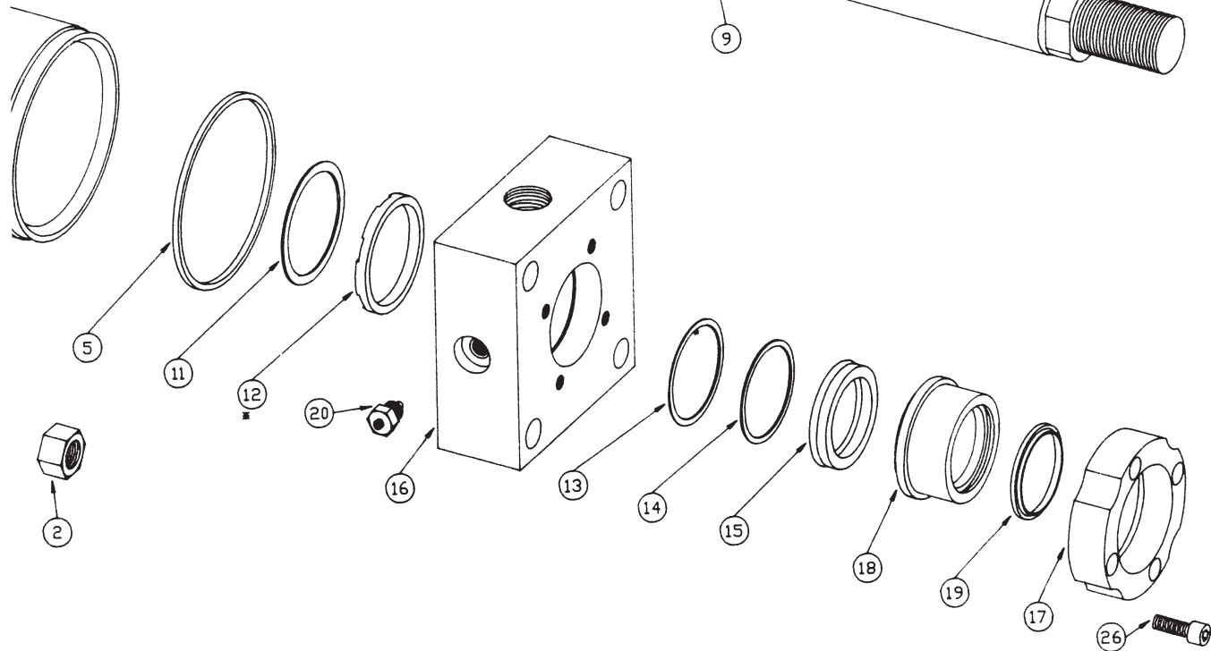
2H STANDARD PISTON (Codes G or H)
