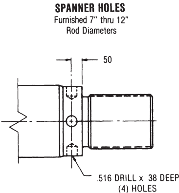
Dimensions are Affected by the Rod Diameter
