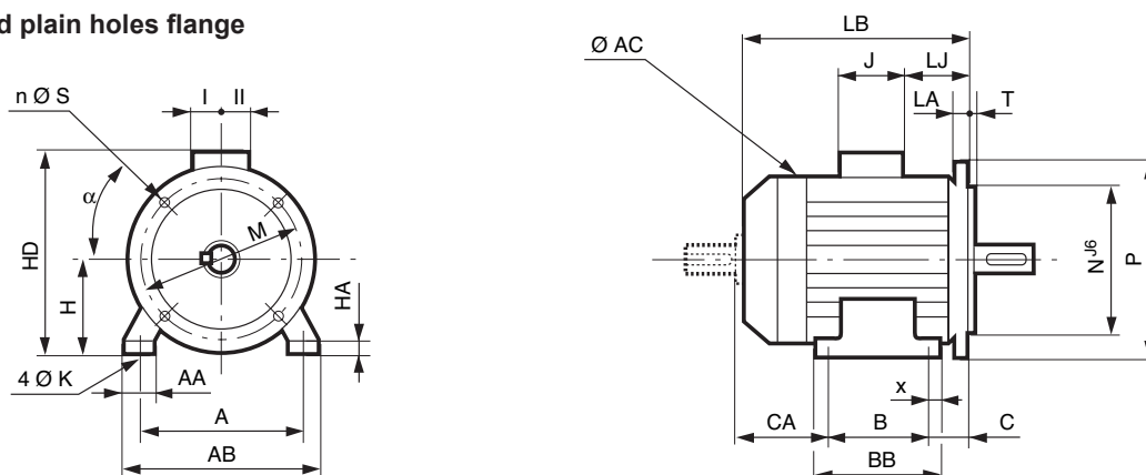
Main dimensions
