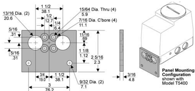
Mounting Bracket: 15268
