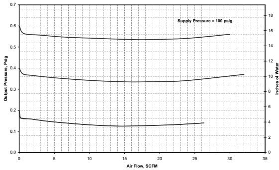
Flow Characteristics Fairchild Model 4114A
