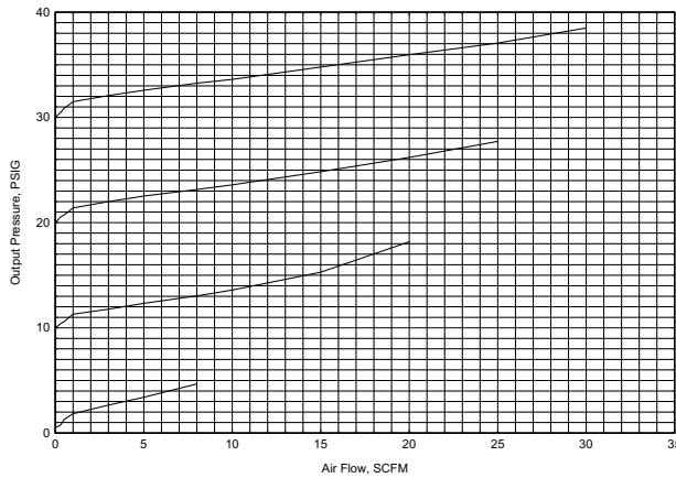
Flow Characteristics Fairchild Model 66232BP
