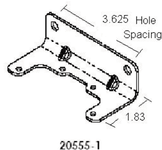
Model 1600A Mounting Bracket Kit P/N 20555-1 zinc plated (sold separately)
