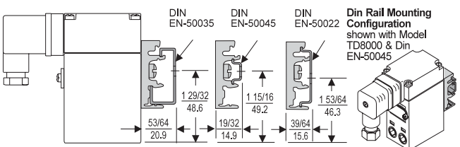
Mounting Bracket: 16893-1
