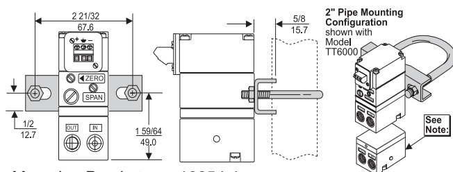
Mounting Bracket: 19254-1
