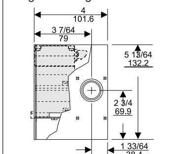
Detail A - Standard Range Front Panel shown with Standard Front Range Mounting Brackets
