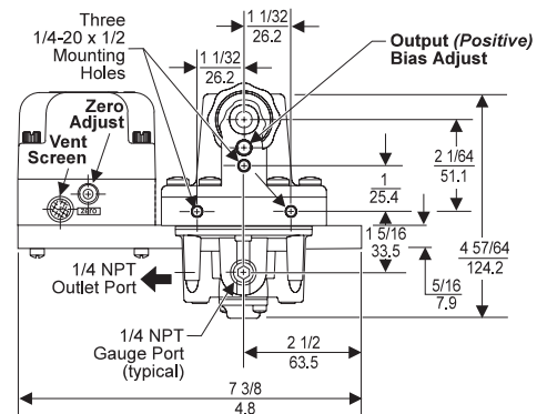
Left View
