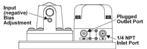
VIEW A
