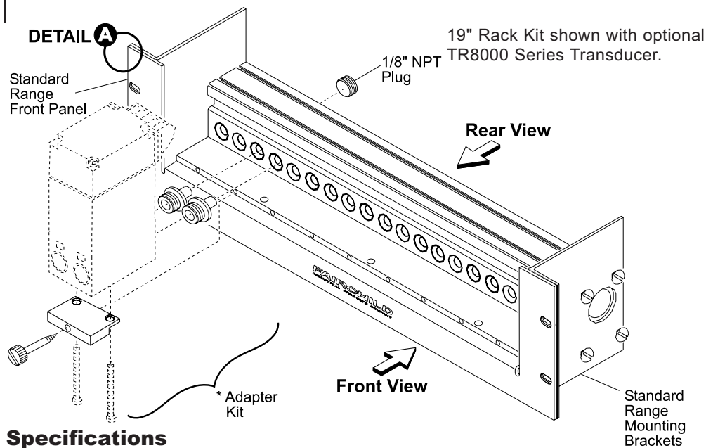
Detail A - Standard Range Front Panel shown with Standard Front Range Mounting Brackets
