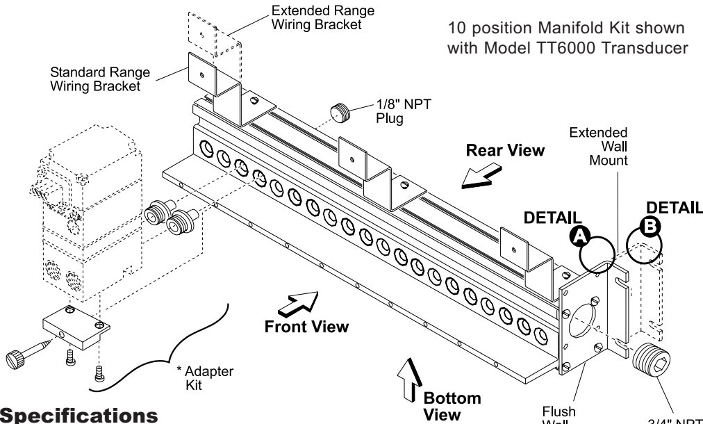
Detail A - Extended Range Unit shown with Flush Wall Mount Bracket.
