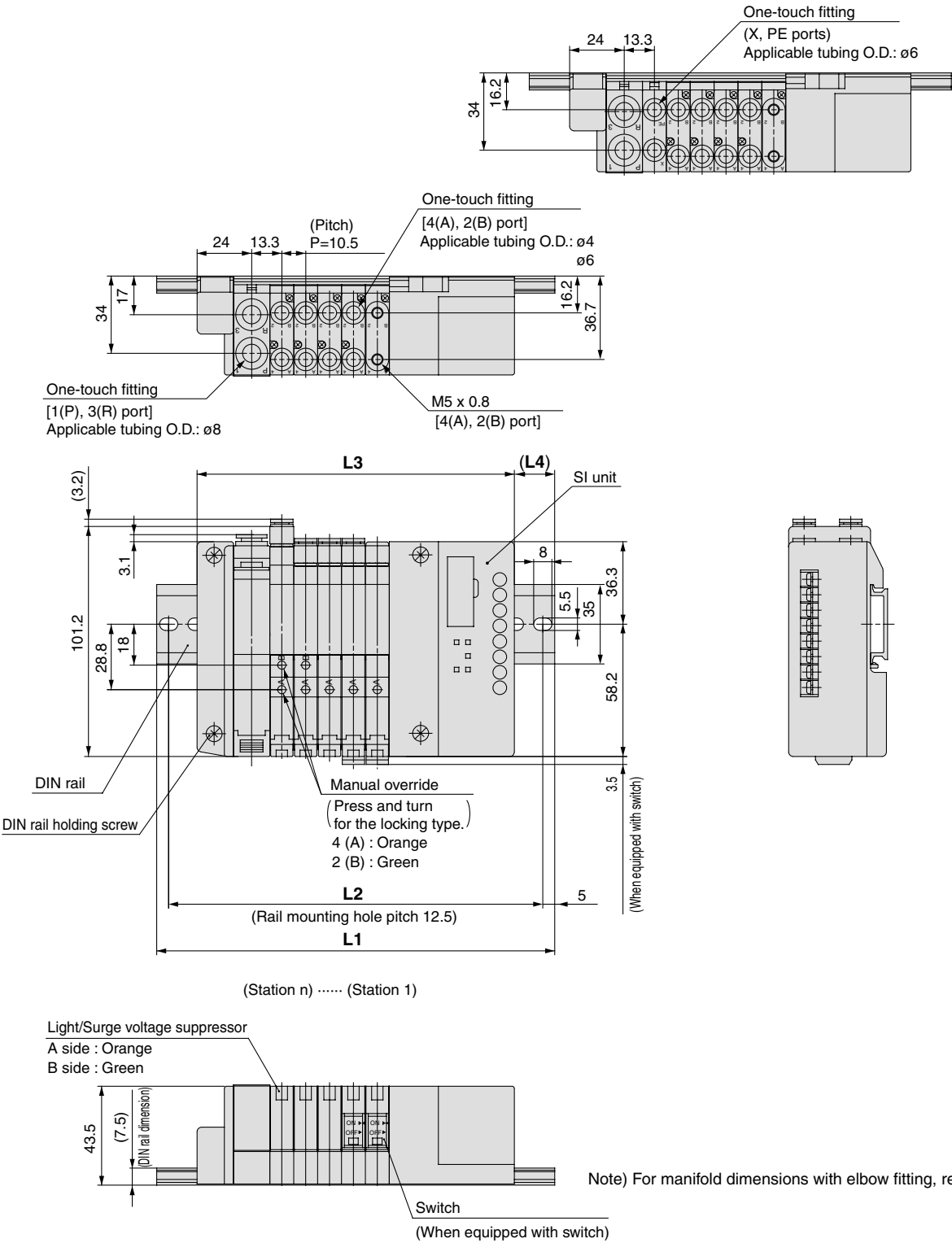
Internal Pilot Manifold L Dimension n : Stations
