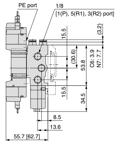
L-type plug connector (L)
