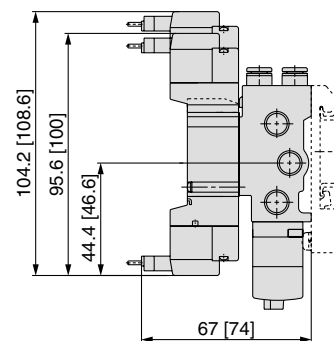
M-type plug connector (M)
