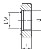
Female BSP Thread (DIN ISO 228)
