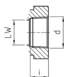
Female NPT Thread (ANSI B1.20.1)
