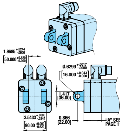
REAR CLEVIS MOUNT (PCD)
