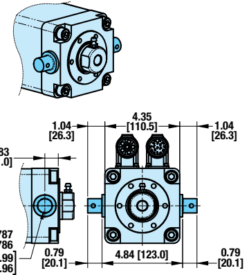
FRONT TRUNNION MOUNT (TRF)
