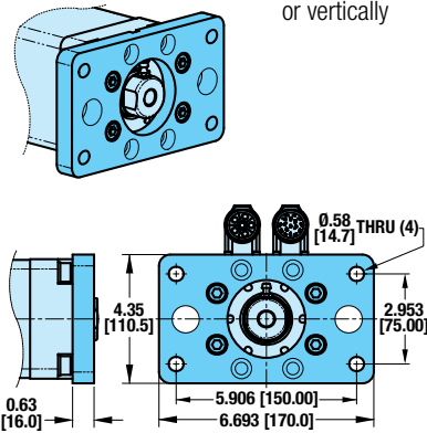
FRONT FLANGE MOUNT (FFG)
