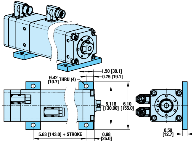
MOUNTING PLATES (MP2)
