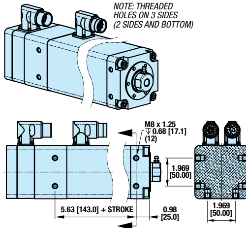
SIDE MOUNTING (MST)
