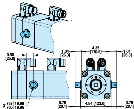
REAR TRUNNION MOUNT (TRR)
