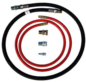
TIM-4431 Connecting Hose Kit for Thunder Oil Pumps Includes 5' air hose, 5' material hose, union adapter, air coupler and connector
