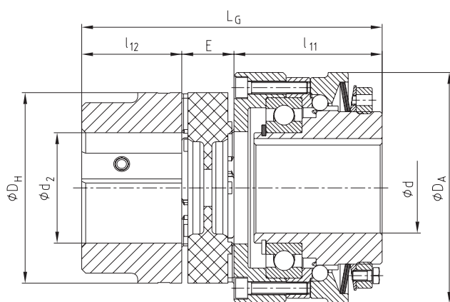
Hub type 1.0
