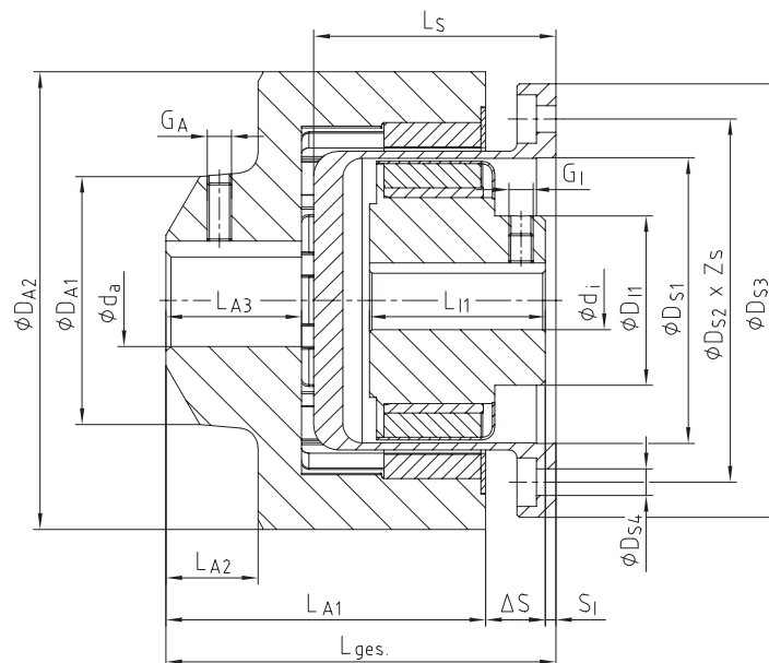
Technical data – Internal rotor and containment shroud
