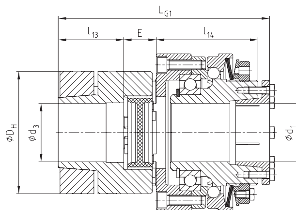
Hub type 6.0
