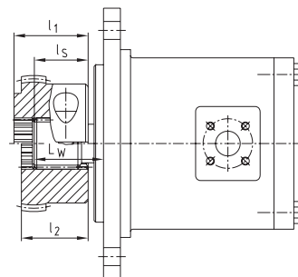
Clamping hub
