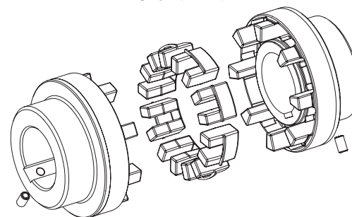
Size 140 - 280
