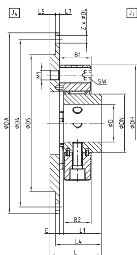
Size 12 - 280
