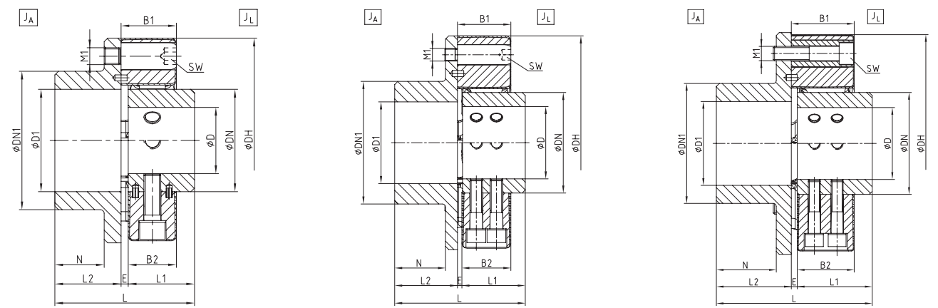
Size 12 - 280
