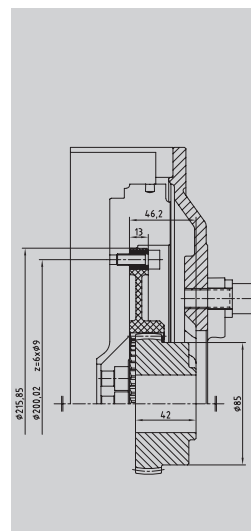
BoWex® T55 FLE-PA Hatz 2-4 H50
