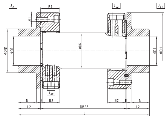
Size 360 - 560
