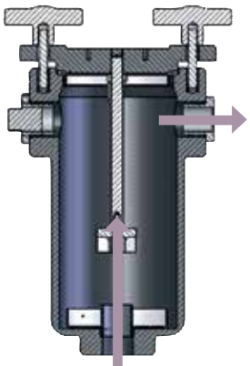
GRAYMILLS INK FILTER
