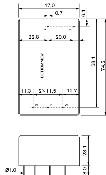
Pinout
