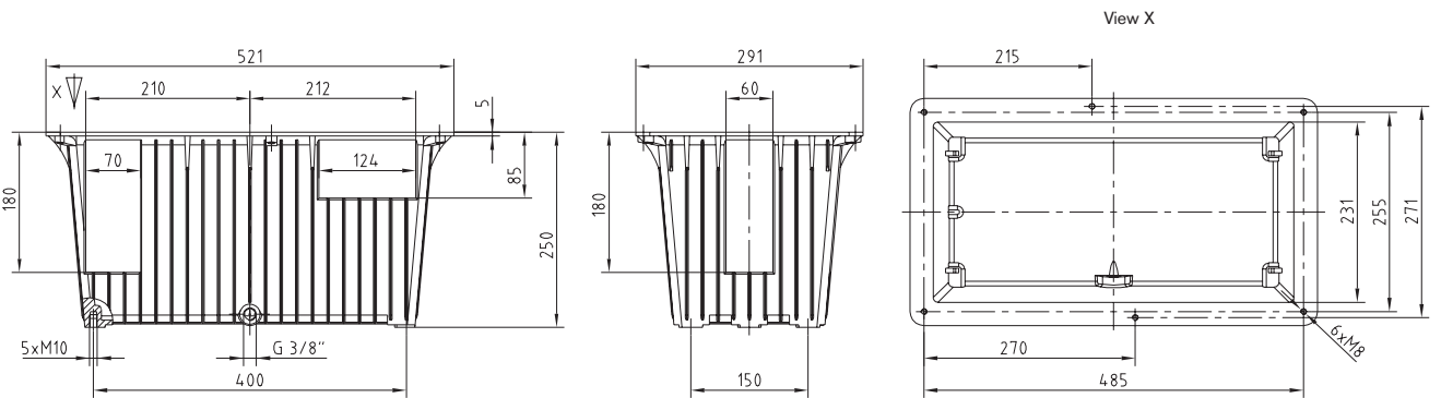
Tank without oil collecting groove BAK 20
