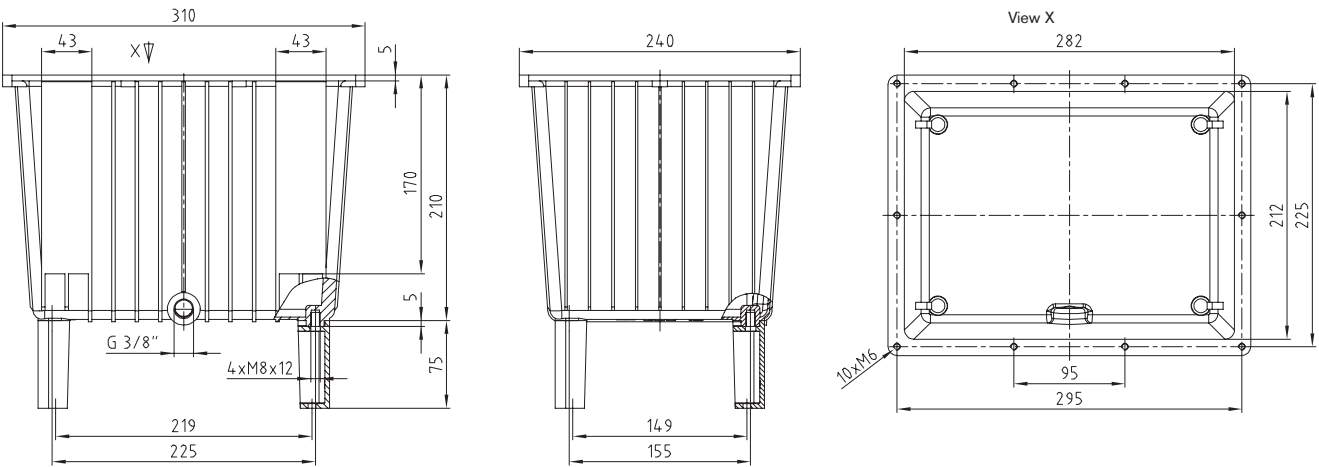
Tank without oil collecting groove BAK 12
