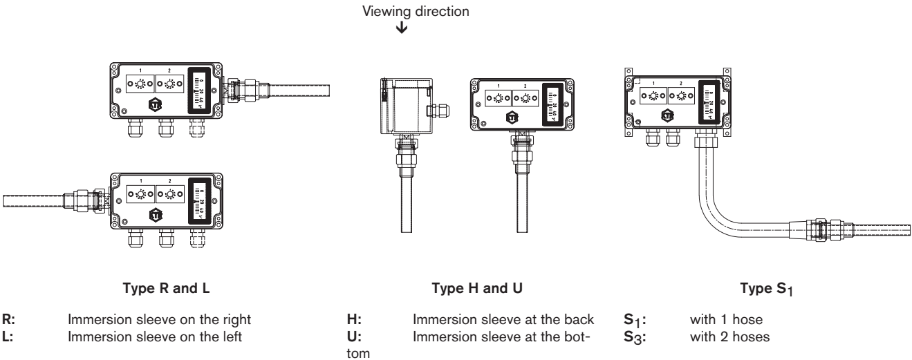
Industrial controller: Type/position of immersion sleeve
