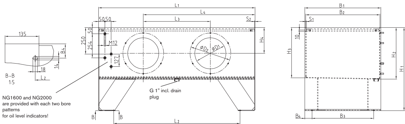
Series BNK design A, NG 63 - 2000
