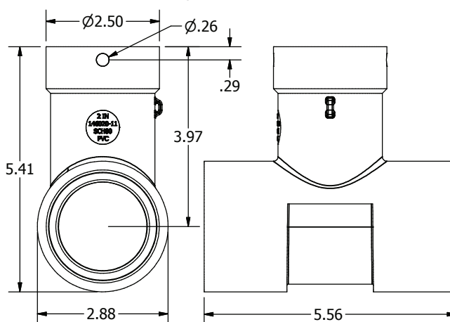
2-INCH Tee Housing
