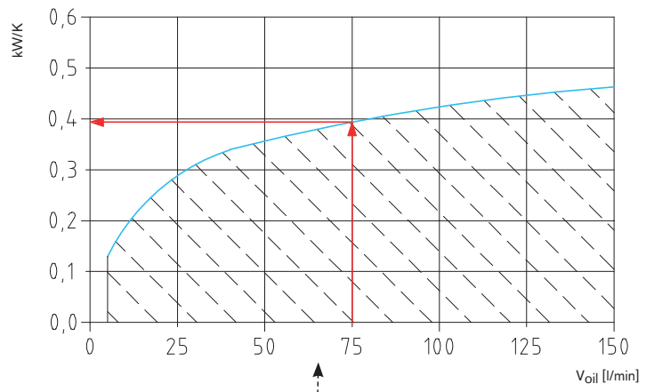
Performance diagramme of OAC400
