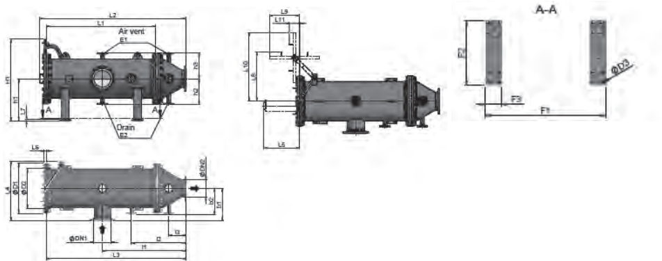
Filter Housing, two-part, carbon steel
