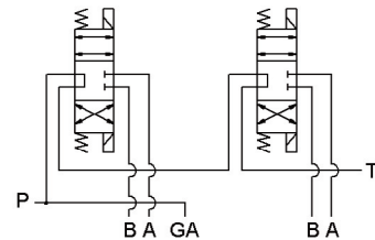
D05 Series circuit
