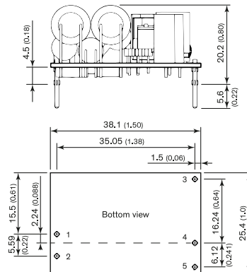
3.3, 5, and 9 VDC models - with heatsink
