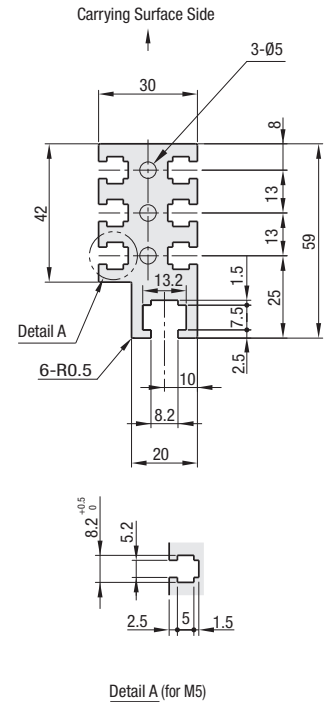
Frame Cross Section and Enlarged View (Symmetrical)
