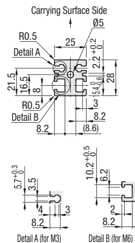
Frame Cross Section and Enlarged View (Symmetrical)
