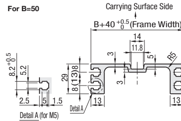
Frame Cross Section and Enlarged View (Symmetrical)
