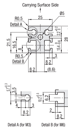
Frame Cross Section and Enlarged View (Symmetrical)
