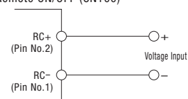
Remote ON/OFF (CN100)
