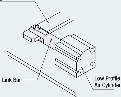
Bearing Embedded Link
