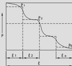
Fig 3. Stepped Load Fluctuation
