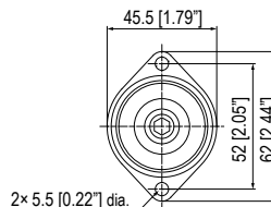
DLW9016/DLW9017
