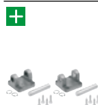
12021-20 Swivel flanges, clevis type for ISO 15552 / 21287
