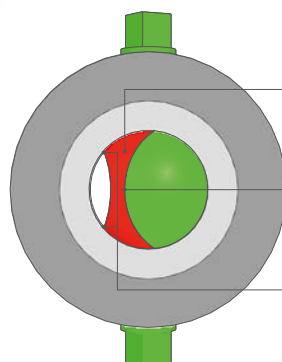
Schubert & Salzer ball sector
