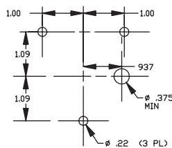
Panel Drill Drawing
