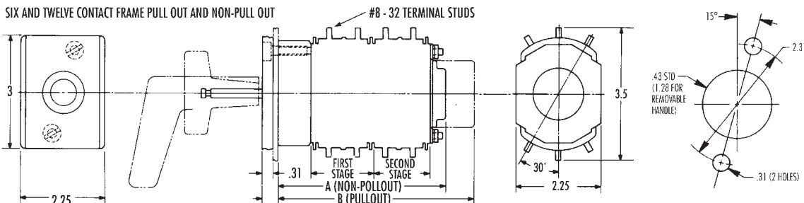
SIX AND TWELVE CONTACT FRAME PULL OUT AND NON-PULL OUT
