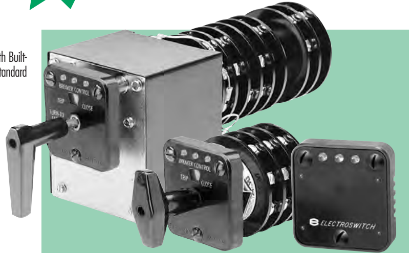
Examples of "Smart" Lighted Nameplate Switches and the Matching Lighted Indicator Nameplate
