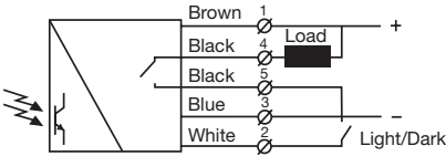
SGR 10 (load as NPN)
