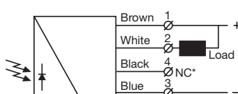
*Do not connect black wire SMR 76xx (load as NPN)
