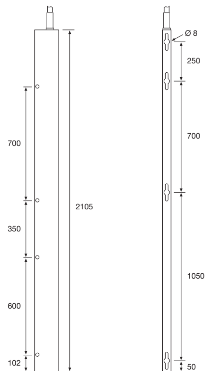
SGT/SGR Side View
