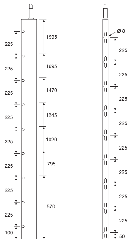
SGT/SGR Side View
