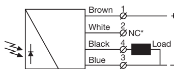
*Do not connect white wire SMR 76xx (load as PNP)
