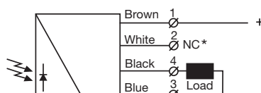
SPR 2645 (load as PNP)
