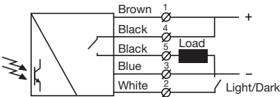
SGR 10 (load as PNP)
