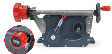
Microdial Control
