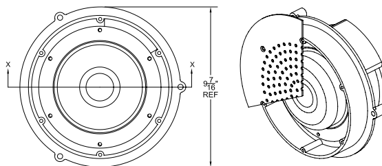
FRONT VIEW (grill not shown for clarity)
