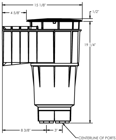
U3 Skimmer for concrete
