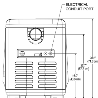
EXHAUST SIDE
